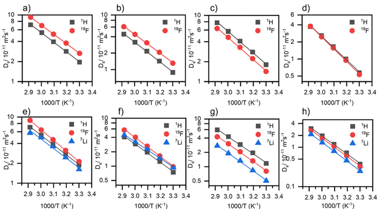
Fig. 6 Temperature dependent self-diffusion coefficients ( ^1\text{H} : IL cation, ^{19}\text{F} : anion, ^7\text{Li} : lithium cation) of neat ILs on top row in order (a) [\text{C}_{101}\text{mpip}][\text{FSI}] , (b) [\text{C}_{101}\text{mmor}][\text{FSI}] , (c) [\text{C}_{101}\text{mpip}][\text{TFSI}] , (d) [\text{C}_{101}\text{mmor}][\text{TFSI}] and their electrolyte solutions directly below, in temperature range 30–70 °C. Errors are within the size of the data points.
