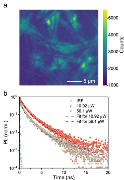
Fig. 3 (a) Microscopy-PL image of BiSBr thin film sample. The bright-field optical micrograph and PL map of the sample were taken over exactly the same area. The optical micrograph is in black and white, while the PL map is shown in color, with the intensity of PL represented by the colorscale displayed. The PL map is superimposed over the optical micrograph. (b) Confocal microscopy-time-correlated single photon counting (TCSPC) measurements of BiSBr in air at 10.9 \mu W and 56.9 \mu W excitation laser power, along with the instrument response function (IRF) and fitted models (refer to Tables S5 and S6, ESI† for details). The excitation wavelength was 520 nm, with a repetition rate of 5 MHz, incident on the film side.
