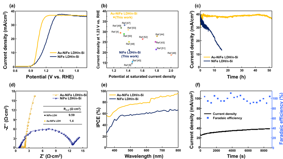
Fig. 3 PEC performances of Au-NiFe LDH/n-Si and NiFe LDH/n-Si photoanodes under AM 1.5G sunlight (100 mW cm -2 ). (a) J – V curves of Au and NiFe LDH based silicon photoanodes in 1 M NaOH aqueous solution. (b) Comparison of photocurrent density at water oxidation potential (1.23 V vs. RHE) and potential to reach saturated photocurrent density with those of previously reported n-Si based photoanodes. (c) Stability tests of photoanodes in buffered NaOH aqueous solution. (d) EIS spectra and (e) IPCE curves of Au-NiFe LDH/n-Si and NiFe LDH/n-Si photoanodes in 1 M NaOH aqueous solution. (f) Faradaic efficiency and the corresponding chronoamperometric curve of the Au-NiFe LDH/n-Si photoanode in 1 M NaOH electrolyte.
