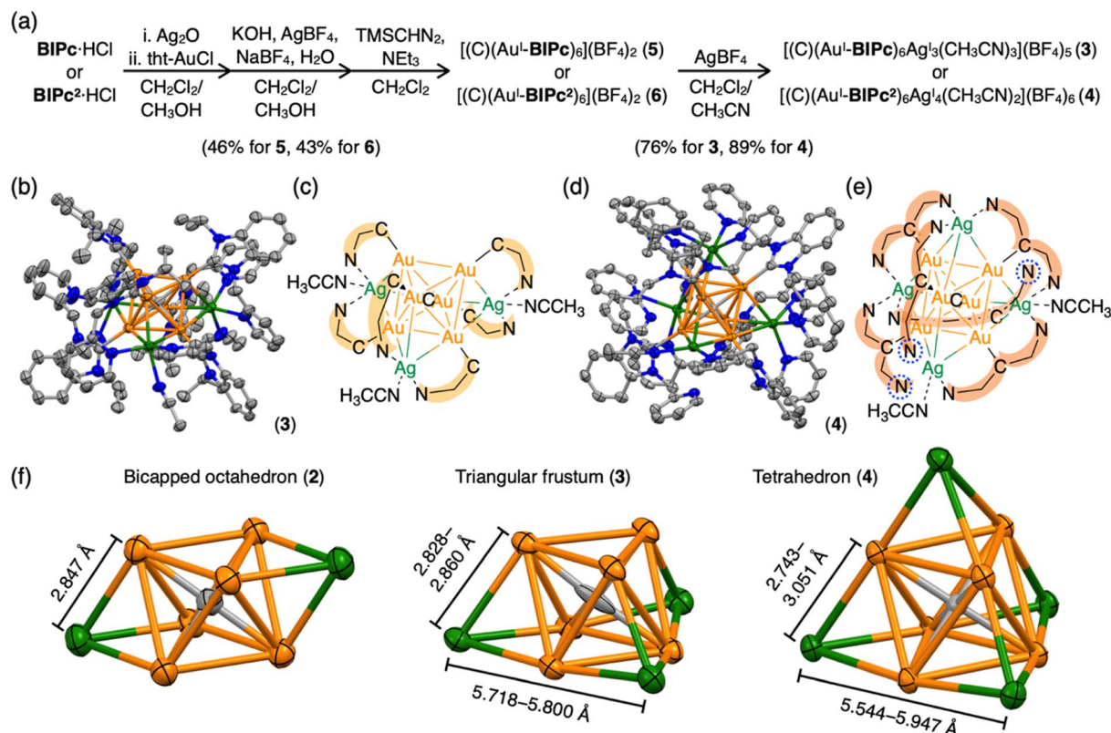
Fig. 2 (a) Synthetic schemes of the homometallic clusters [(C)(Au^I-BIPc)_6](BF_4)_2 ( 5 ) and [(C)(Au^I-BIPc^2)_6](BF_4)_2 ( 6 ), and heterometallic clusters [(C)(Au^I-BIPc)_6Ag_3^I(CH_3CN)_3](BF_4)_5 ( 3 ) and [(C)(Au^I-BIPc^2)_6Ag_4^I(CH_3CN)_2](BF_4)_6 ( 4 ). (b) Molecular structure of cluster 3 . (c) A simplified scheme showing the structure of cluster 3 . C ∧ N represents ligand BIPc . (d) Molecular structure of cluster 4 . (e) A simplified scheme showing the structure of cluster 4 . N ∧ C ∧ N represents ligand BIPc 2 . Uncoordinated pyridyl groups are highlighted by dashed blue cycles. (f) Comparison of structures of bicapped octahedral CAu_6Ag_2 in cluster 2 , triangular frustum-shaped CAu_6Ag_3 in cluster 3 , and tetrahedral CAu_6Ag_4 in cluster 4 . The length of the edge of each structure is shown.
