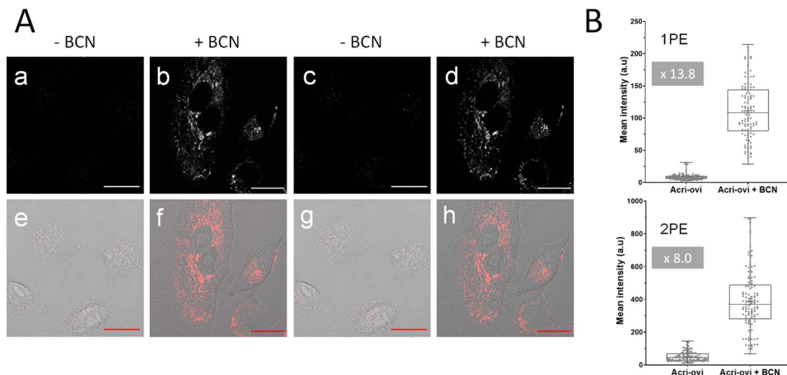
Fig. 7 (A) Confocal microscopy imaging of live A549 cells incubated with Acridine-ovi at 2 \mu\text{M} for 3 h and then with (b and d) or without (a and c) BCN at 50 \mu\text{M} for 30 min under one (496 nm, a and b) or two-photon excitation (840 nm, c and d). (e), (f), (g) and (h) The corresponding merged images (fluorescence and brightfield). Emission slit settings: 500–700 nm. Scale bar: 20 \mu\text{m} . (B) Fluorescence quantification in live A549 cells with Acridine-ovi (2 \mu\text{M} ) and BCN (10 \mu\text{M} ). Box plot represents the fluorescence intensity obtained by measuring pixel means using ImageJ software under one (1PE) (up) or two-photon excitation (2PE) (down). Data come from three independent experiments, and settings and processing were identical for all images. **** p < 0.0001 .
