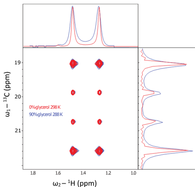
Fig. 5 In order to simulate the rotational environment of the labelled amino acid inside a protein, \text{L-}[\alpha\text{-}^2\text{H}, ^{15}\text{N}, \beta\text{-}^{13}\text{C}]\text{-alanine} was dissolved in a viscous glycerol medium and studied by NMR. The figure shows the ^{13}\text{C}\text{-}^1\text{H} decoupled HSQC experiment of the sample in ^2\text{H}_2\text{O} at 298 K (red) and 90 vol% glycerol at 288 K (blue trace). Under 0 vol% glycerol, the ratio of intensities is 3 : 1 : 1 : 3, as expected for a small molecule. At 90 vol% glycerol and low temperature, the resonances remained intense. The intensity ratio changed to approximately 2 : 1 : 1 : 2. Due to the outer resonances having 9\times faster relaxation than the inner lines, in the macromolecular limit when the molecule tumbles slowly. Although the effects of slow tumbling are clear, the resonances remain sharp indicating the utility of this reagent inside high molecular weight proteins.
