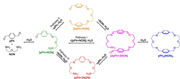
Scheme 2 Stepwise [2 + 2] imine condensation processes showing the intermediates on the way to the formation of the imine-based dynamic covalent macrocycle pPh_2(NON)_2 .
