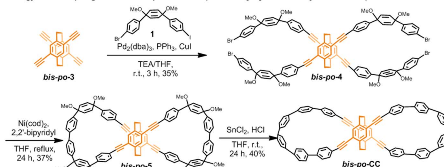
Strategy A: One step ring closures at the pseudo-ortho position of [2.2]PCP for the synthesis of bis-po-CC
