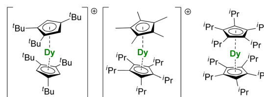
Fig. 8 Molecular structures [Dy(Cp^{ttt})_2]^+ , 72,73 [Dy(Cp^*)_2(Cp^{iPr5})]^+ , 74 and Dy(Cp^{iPr5})_2 . 193
