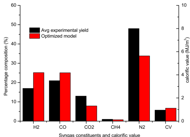
Fig. 10 Comparison final gas output and calorific value of optimized gasifier model with average experimental yield.
