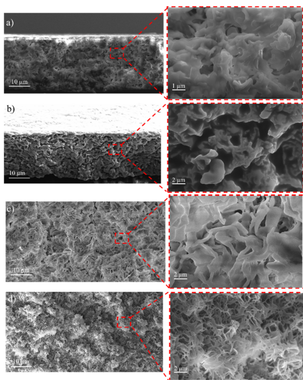
Fig. 3 Cross-sections of the HDPE membranes: (a) R-HDPE 8%, (b) R-HDPE 10%, (c) R-HDPE 13%, and (d) R-HDPE 15%.
