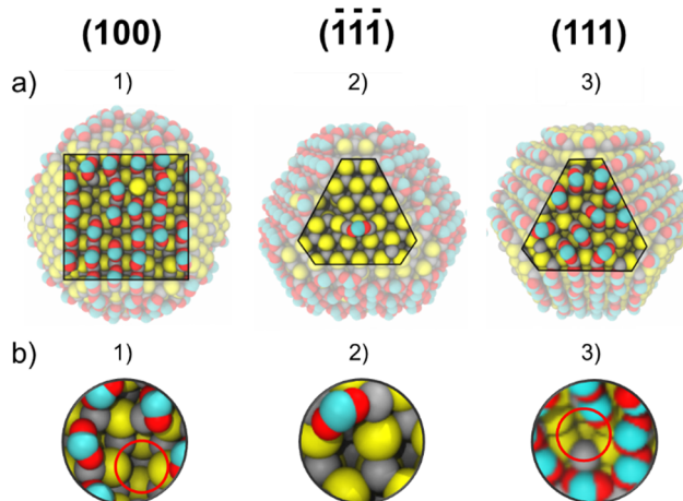
Fig. 4 (a) Structural representations and (b) details of the packing of the oleate ligands on the different facets of the NC model for: (1) facet (100), (2) facet (111) and (3) facet (111). Cd vacancies are circled in red.
