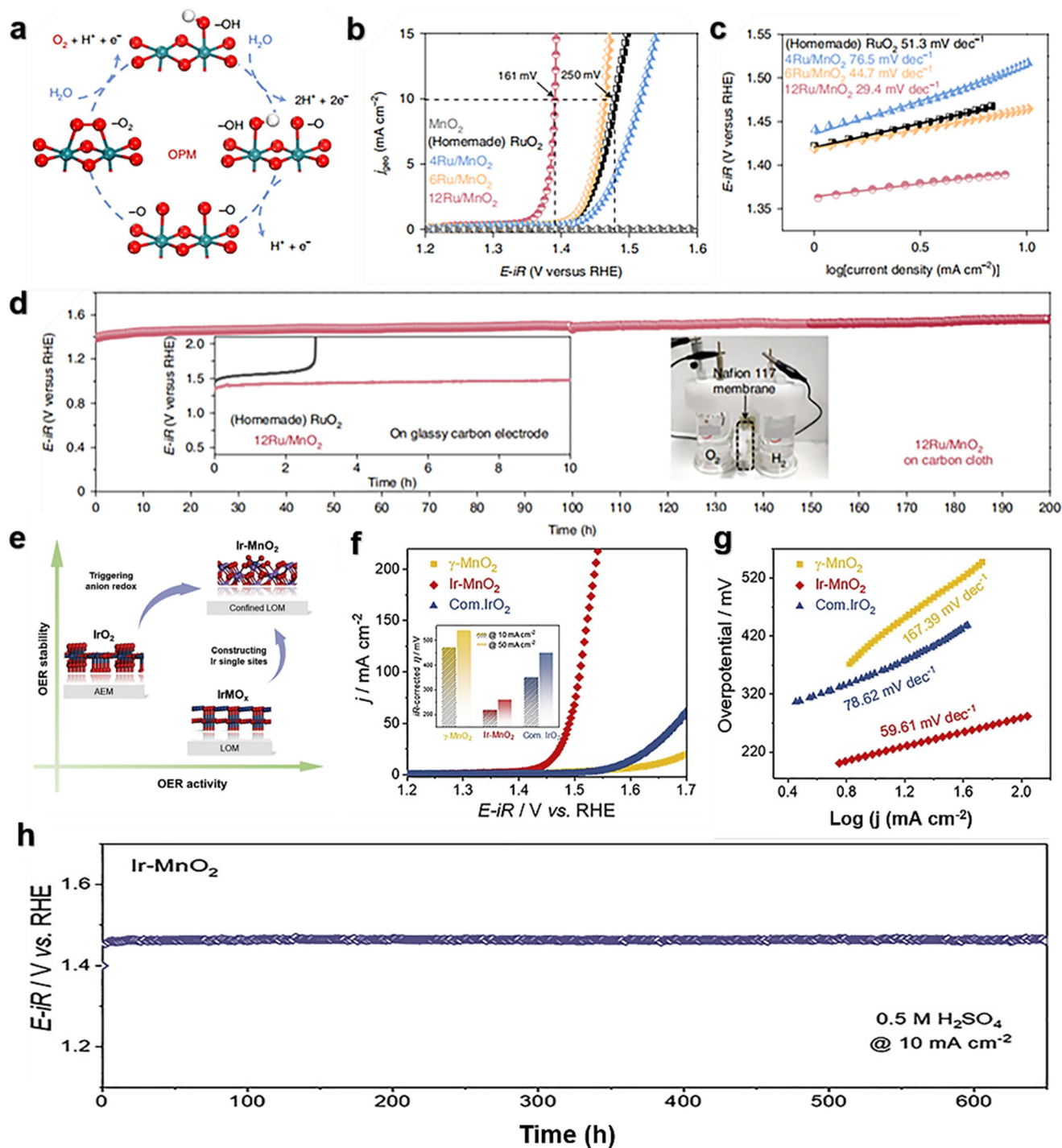
Fig. 6 (a) Oxide path mechanism (OPM); (b) electrocatalytic OER performance of MnO_2 , Ru/MnO_2 and homemade RuO_2 in 0.1\text{ M HClO}_4 ; (c) Tafel slopes of MnO_2 , Ru/MnO_2 and homemade RuO_2 ; (d) chronopotentiometric response of the 12Ru/MnO_2 catalyst. Reprinted with permission from ref. 89. Copyright 2021, Nat. Catal. (e) The design of an Ir single-atom catalyst can trigger lattice oxygen oxidation locally while maintaining the stability of the bulk structure; (f) representative LSV curves of MnO_2 , Ir-MnO 2 , and commercial IrO 2 in 0.5\text{ M H}_2\text{SO}_4 ; (g) Tafel slope of MnO_2 , Ir-MnO 2 , and IrO 2 ; (h) chronopotentiometric response of Ir-MnO 2 for the OER at 10\text{ mA cm}^{-2} . Reprinted with permission from ref. 90. Copyright 2021, Joule .
