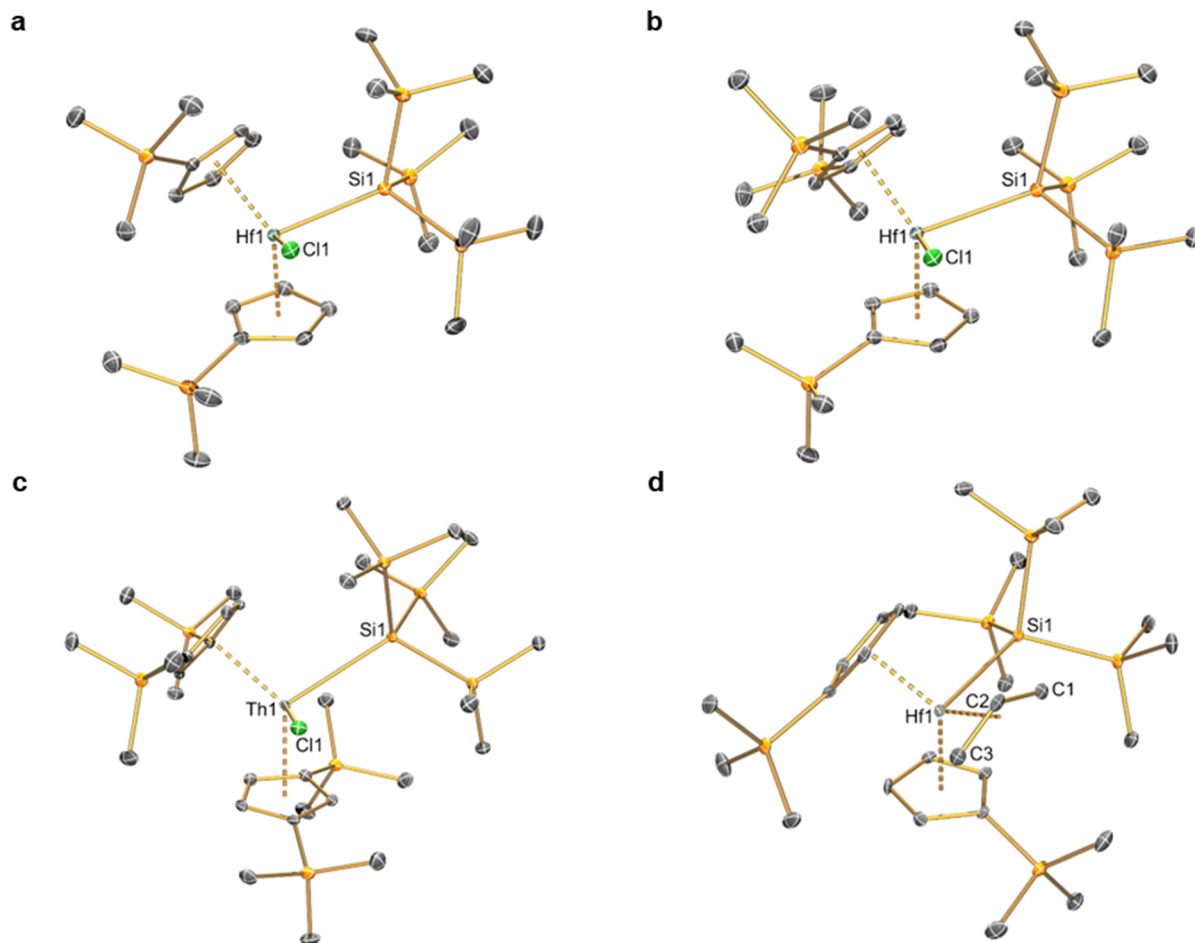
Fig. 1 Single crystal XRD structure of (a) [\text{Hf}(\text{Cp}')_2\{\text{Si}(\text{SiMe}_3)_3\}(\text{Cl})] ( 2 ), (b) [\text{Hf}(\text{Cp}'')(\text{Cp})\{\text{Si}(\text{SiMe}_3)_3\}(\text{Cl})]\cdot 0.5\text{C}_5\text{H}_{12} ( 3·0.5C 5 H 12 ), (c) [\text{Th}(\text{Cp}'')_2\{\text{Si}(\text{SiMe}_3)_3\}(\text{Cl})] ( 4 ) and (d) [\text{Hf}(\text{Cp}')_2\{\text{Si}(\text{SiMe}_3)_3\}(\eta^3\text{-C}_3\text{H}_5)] ( 5 ) with selective atom labelling. Displacement ellipsoids set at 30% probability level and hydrogen atoms, lattice solvent and modelled disorder components omitted for clarity.
