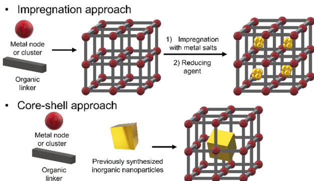
Fig. 5 Schematic representation of different approaches to produce inNPs@NMOFs nanocomposites.
