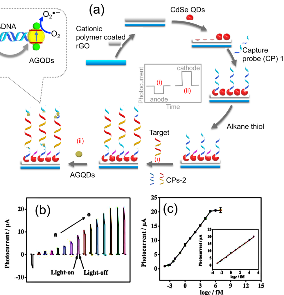
Fig. 9 (a) Schematic illustration of DNA-associated Z-scheme CdSe QDs/AGQDs CdSe for the PEC sensing of T-DNA, (b) photocurrent signals generated by the PEC sensor against varying T-DNA concentrations, such as 0, 0.1 aM to 10 nM (shown with an arrow from a → o) and (c) plot showing the relationship between the photocurrent value and the T-DNA analyte concentration. The inset shows the linearity for varying concentrations (fM) against the photocurrent in terms of \mu\text{A} . 87 (a–c reprinted with permission from ref. 87 copyright © 2019 Elsevier B.V.)
