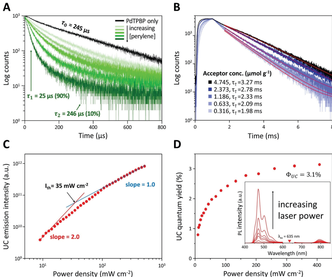
Fig. 3 (A) Phosphorescence lifetimes of PdTPBP with increasing concentrations of perylene ([PdTPBP] = 0.03 \mu mol g^{-1} and [perylene] = 0 – 4.7 \mu mol g^{-1} in PCL). (B) UC emission decay profiles of the UC PCL at 470 nm following excitation at 635 nm ([PdTPBP] = 0.03 \mu mol g^{-1} and [perylene] = 0 – 4.7 \mu mol g^{-1} in PCL). (C) Integrated UC emission intensity and (D) UC quantum yields of the UC PCL as a function of the power density of 635 nm laser excitation ([PdTPBP] = 0.03 \mu mol g^{-1} and [perylene] = 4.7 \mu mol g^{-1} in PCL). The inset in (D) shows UC emission spectra of UC PCL with increasing 635 nm laser excitation. A 632 nm notch filter was used to eliminate the scattered incident light.
