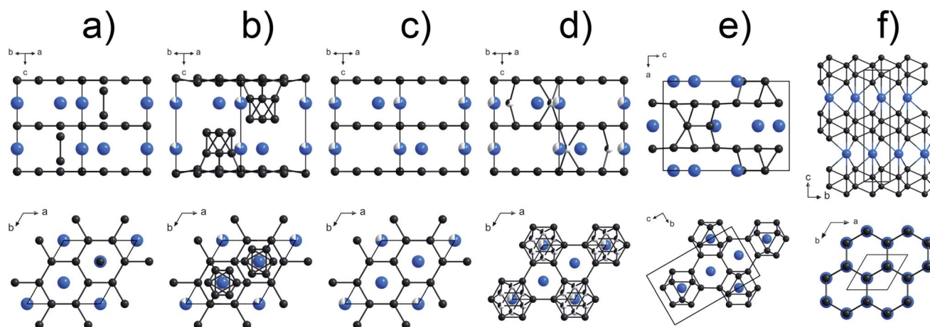
Fig. 1 Various models of the crystal structure proposed for WB 4 : (a) the crystal structure of WB 4 by Romans and Krug; 39 (b) W 1.83 B 9 by Nowotny et al. 58 (c) W 1–x B 3 following Lundström and Rosenberg 59 and Zeiringer et al. 42 (d) WB 4.2 by Lech et al. 47 (e) WB 5 by Kvashnin et al. 34,54 (f) theoretically predicted stoichiometric WB 4 . 31,36,37,48 The blue spheres represent tungsten atoms, the black spheres are boron atoms, and the partially filled spheres indicate defect B or W sites.
