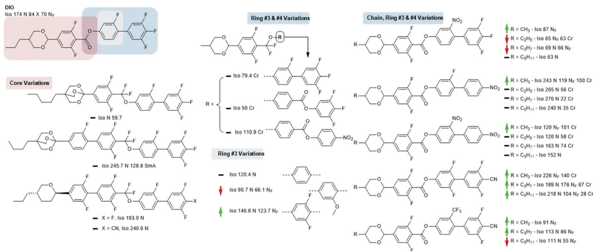
Fig. 5 Structural variants of DIO; transition temperatures (°C) are on cooling from the isotropic liquid. 28,31–33 Green and red arrows indicate increased and decreased T NF–N relative to the parent material, respectively, while a black dash indicates the absence of the N F phase.
