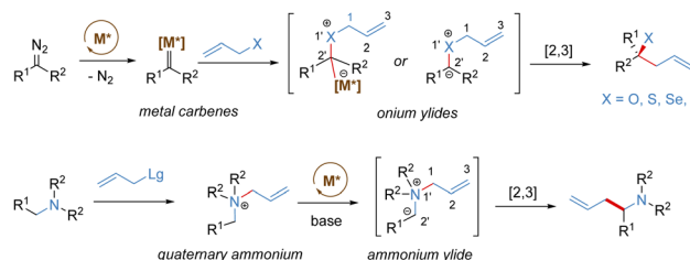
Scheme 16 Metal-catalysed asymmetric [2,3]-sigmatropic rearrangements.
