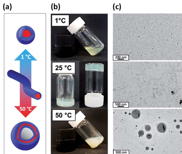
Fig. 2 (a) Schematic representation of the reversible morphological transitions exhibited by a 20% w/w aqueous dispersion of 'shape-shifting' PDMAC 49 -P(HBA-stat-DAAM) 302 nano-objects on varying the temperature from 1 °C to 50 °C. (b) Digital photographs illustrating the change in physical appearance of a 20% w/w aqueous dispersion of PDMAC 49 -P(HBA-stat-DAAM) 302 nano-objects recorded at 1 °C, 25 °C and 50 °C (after allowing 30 min for thermal equilibrium at each temperature). (c) Corresponding TEM images recorded for 0.10% w/w aqueous dispersions of the same PDMAC 49 -P(HBA-stat-DAAM) 302 nano-objects after their covalent stabilization at the desired temperature using a disulfide-based adipic acid dihydrazide [DS-ADH] crosslinker at a DS-ADH/DAAM molar ratio of 0.50 (spheres crosslinked at 1 °C, worms crosslinked at 25 °C, and vesicles crosslinked at 50 °C).
