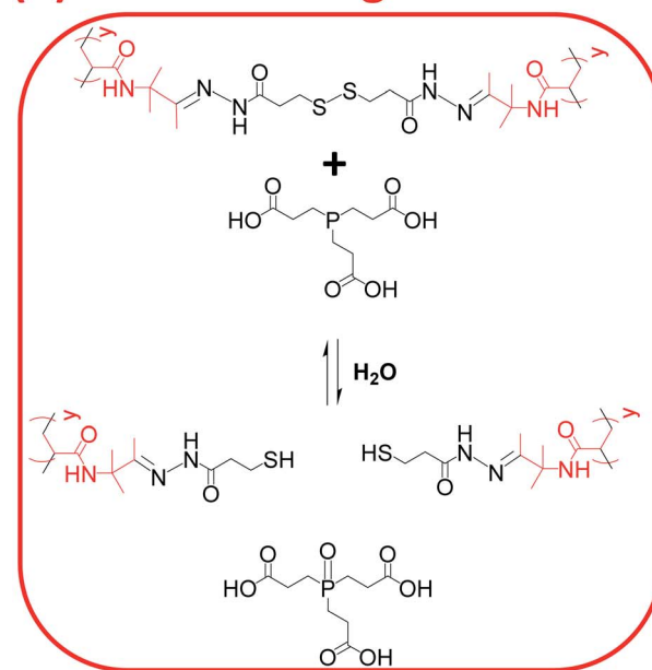
Scheme 2 (a) Nucleophilic attack of pendent ketone groups on DAAM repeat units by DS-ADH, which leads to crosslinks between the hydrophobic P(HBA-stat-DAAM) 302 chains. (b) Reductive cleavage of disulfide bonds within these crosslinks using tris(2-carboxyethyl) phosphine (TCEP).
