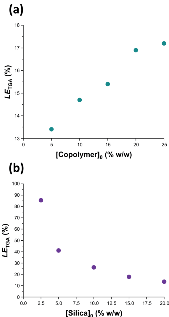
Fig. 6 Vesicle loading efficiency, LE_{TGA} , as determined by thermogravimetric analysis for: (a) a series of silica-loaded PDMA 49 -P(HBA- stat -DAAM) 302 vesicles prepared at various copolymer concentrations using a constant silica nanoparticle concentration of 20% w/w; (b) a series of PDMA 49 -P(HBA- stat -DAAM) 302 vesicles prepared at various silica nanoparticle concentrations using a constant copolymer concentration of 10% w/w. See Section 2.1 of the ESI† for further details of the LE_{TGA} calculation.
