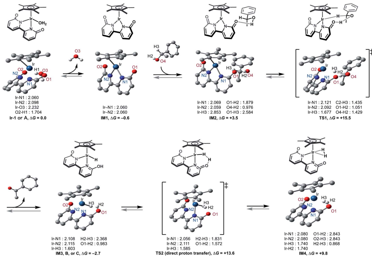
Fig. 5 Geometry and energy changes of the proposed pathway at the CAM-B3LYP + GD3 level of theory using SDD and 6-31+G** basis sets for Ir and other atoms, respectively. Solvent effect ( \text{H}_2\text{O} ) by IEPCM method; Gibbs free energies in \text{kcal mol}^{-1} at T = 353.15 \text{ K} .
