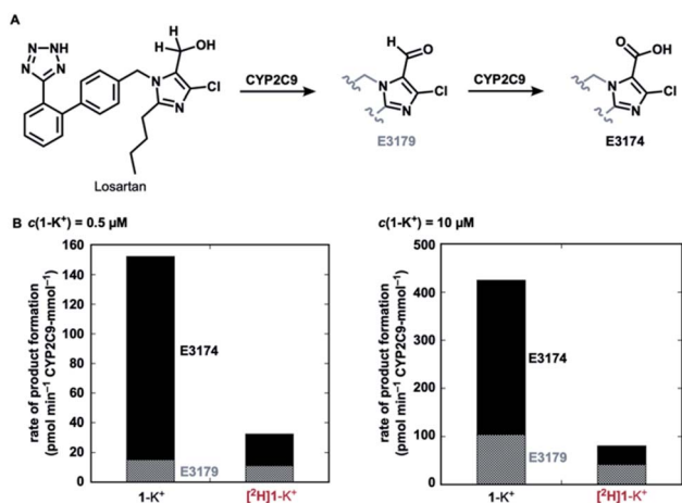
Fig. 6 (A) Metabolic pathway of losartan and (B) kinetic data on the formation of metabolites E3179( -d_1 ) and E3174 from 1\text{-K}^+ or [ ^2\text{H} ] 1\text{-K}^+ (96% D ) by CYP2C9 under non-competitive intermolecular conditions.
