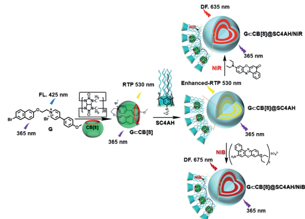
Fig. 15 Schematic illustration of the construction of light-harvesting phosphorescence energy transfer supramolecular assembly via SC4AH, CB[8], and bromonaphthalene-modified methoxypyridine.
