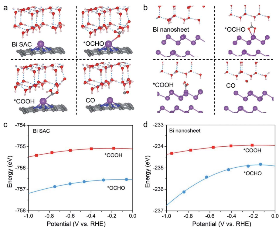
Fig. 1 Geometric structures of the 2\text{e}^- \text{CO}_2\text{RR} species for (a) the Bi-N-C SAC and (b) the Bi nanosheets. The violet, grey, red, and white spheres denote Bi, C, O, and H, respectively. The blue dashed lines indicate the hydrogen bond. Computed total energies of ^*\text{OCHO} and ^*\text{COOH} on (c) the Bi-N-C SAC and (d) the Bi nanosheets as a function of potential.
