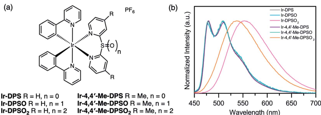
Fig. 16 (a) Structures of Ir(III) complexes Ir-DPSO n and Ir-Me-DPSO n ( n = 0-2 ) reported by our group. (b) PL spectra of the Ir(III) complexes in \text{CH}_2\text{Cl}_2 solution ( \lambda_{\text{ex}} = 390 \text{ nm} ). Adapted with permission from ref. 82. Copyright 2017 American Chemical Society.
