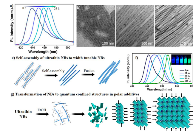
Fig. 8 (a) PL emission of ultrathin NBs upon the continuation of reaction for several hours; corresponding TEM images are presented in (b) to (d). (e) Schematic illustration of the RT growth profile of NBs from lamellar-type Cs–Pb–Br structures to 9 nm NBs. (f) PL emission of ethanol-induced growth of NBs to NCs and corresponding photographs under UV light. (g) Schematic illustration of the transformation of NBs in the presence of ethanol resulting in ligand destabilization on the NB surface and followed by proactive growth.
