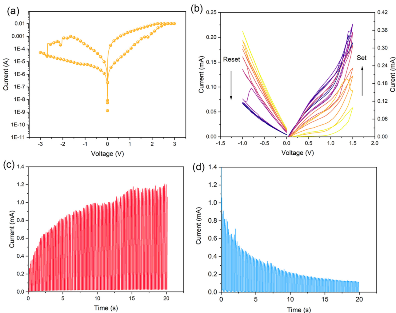
Fig. 2 (a) Typical current–voltage ( I – V ) curve of the \text{AgBiI}_4 artificial synapse under positive and negative sweeps. (b) I – V curves under 10 positive and 10 negative voltage sweeps ( 0 \rightarrow 1.5 \rightarrow 0 \rightarrow -1.0 \rightarrow 0 V). (c) The EPSC plasticity with positive pulses ( 1.5 V, 0.1 s). (d) The EPSC plasticity with negative pulses ( -1.5 V, 0.1 s).
