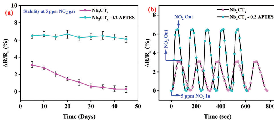
Fig. 8 (a) Long-term stability and (b) repeatability of \text{Nb}_2\text{CT}_x and \text{Nb}_2\text{CT}_x -0.2 APTES-based \text{NO}_2 gas sensor.
