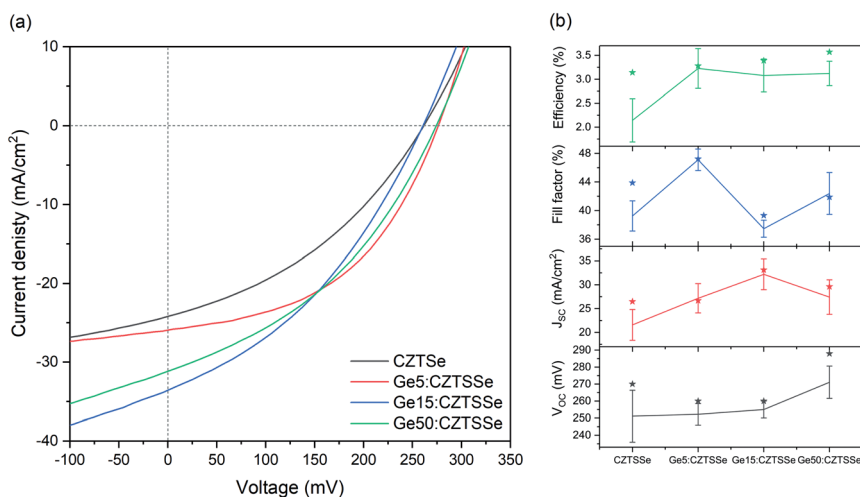
Fig. 6 CZTSSe device performance (a). J – V characteristics under a simulated AM1.5G spectrum and (b) statistical analysis of the performance parameters: V_{\text{OC}} , J_{\text{SC}} , fill factor and conversion efficiency, showing the standard deviation.
