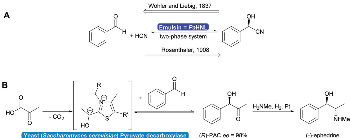
Scheme 1 (A) In 1837 Wöhler and Liebig described the PaHNL-catalysed degradation of ( R )-mandelonitrile. In 1908 Rosenthaler reversed this reaction in the synthesis direction, the first enantioselective reaction described. (B) Since the 1930s the industrial synthesis of L-ephedrine is based on the yeast-catalysed enantioselective synthesis of ( R )-PAC.
