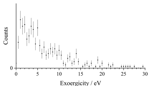
Fig. 7 Experimental exoergicity spectrum for the dissociation of \text{H}_2^{+} to form \text{H}^+ + \text{H} . The \text{H}_2^{+} is formed via the initial electron-transfer reaction \text{S}^{2+} + \text{H}_2 \rightarrow \text{S}^+ + \text{H}_2^{+*} . The error bars represent two standard deviations of the counts. See text for details.
