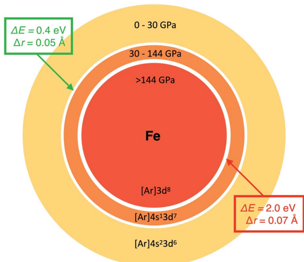
Fig. 3 Example of the relationship between atomic radius and total energy. The size of the Fe atom at different pressures is to scale. White regions correspond to [Ar]4s²3d⁶ ( S = 2 ) \rightarrow [Ar]4s¹3d⁷ ( S = 2 ) and [Ar]4s¹3d⁷ \rightarrow [Ar]3d⁸ ( S = 1 ) ground state configurational transitions predicted at 30 and 144 GPa, respectively.
