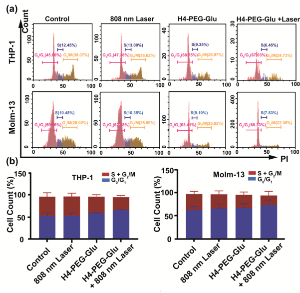
Fig. 4 (a) Flow cytometry analysis of the cell cycle of THP-1 and Molm-13 cells treated with PBS, H4-PEG-Glu (20 \mu M), and H4-PEG-Glu (20 \mu M) under 808 nm laser irradiation ( 1.2 \text{ W cm}^{-2} , 5 min). (b) Proportions of G_0/G_1 , S, and G_2/M phase cells in THP-1 and Molm-13. * p < 0.05 ; ** p < 0.01 ; *** p < 0.001 ; ns, not significant.
