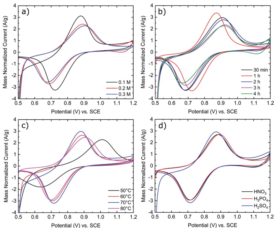
Fig. 2 Mass normalized cyclic voltammograms of K-GF electrodes in 1 : 1 ratio 0.1 M VO 2 + : VO 2 2+ in 2 M H 2 SO 4 with 100 mM H 3 PO 4 solution. CV was conducted at 5 mV s -1 scan rate at room temperature. (a) Variation of KMnO 4 concentration. (b) Variation of immersion time. (c) Variation of solution temperature. (d) Variation of supporting acid. Exact testing conditions of all electrode samples are stated in Table 1.
