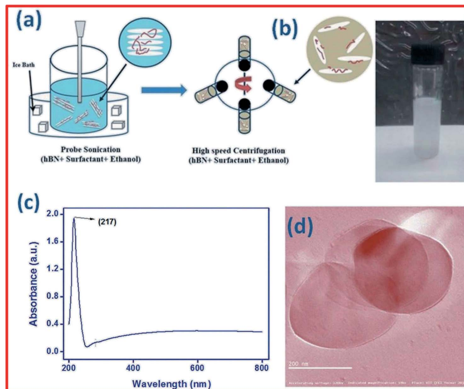
Fig. 15 (a) A schematic diagram of the synthesis of h-BN nanosheets in surfactant solution. (b) An image of the centrifuged solution. (c) The UV-vis-NIR spectrum of h-BN nanosheets. (d) A TEM image of exfoliated BNNSSs. 152
