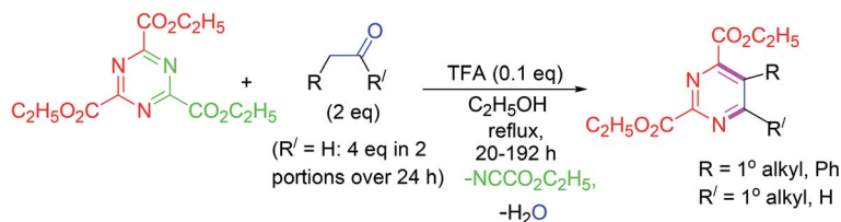
Scheme 15 Synthesis of highly functionalized pyrimidines by IEDDA reaction under TFA catalysis.
