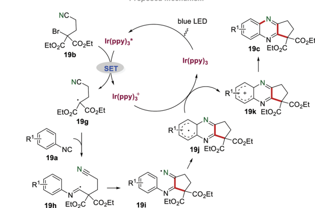
Scheme 19 The synthesis of fused quinoxaline derivatives.
