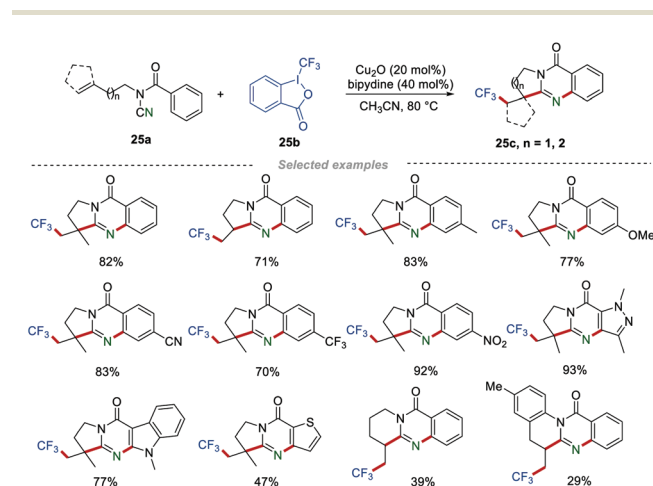
Scheme 25 The preparation of trifluoromethylated quinazolinones.
