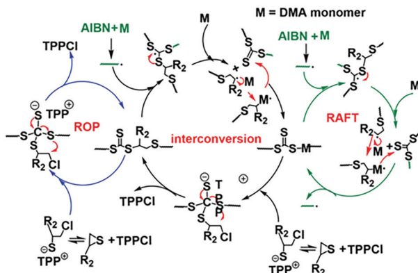
Fig. 4 Interconvertible hybrid copolymerizations of AROP and RAFT. Reproduced from ref. 23 with permission from the Royal Society of Chemistry, copyright 2019.
