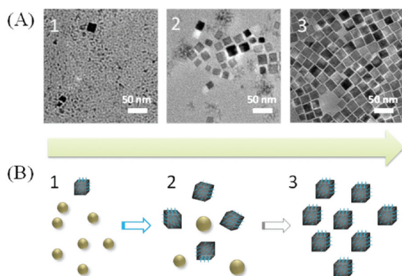
Fig. 14 (A) TEM of the \text{Cu}_3\text{N} NCs synthesized according to ref. 105, after 2, 5 and 10 min. (B) The proposed growth procedure of \text{Cu}_3\text{N} nanocubes. Reproduced from ref. 105 with permission from the Royal Society of Chemistry.
