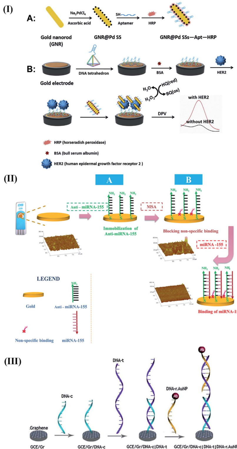
Fig. 2 Different examples of electrochemical biosensing approaches for breast cancer detection. (I) Schematic representation of GNR@Pd SSs—Apt—HRP: formation and its application for HER2 detection. Reproduced with permission. 27 Copyright 2019, Elsevier. (II) Schematics of the steps involved in the electrochemical detection of mi-RNA 155. Reproduced with permission. 35 Copyright 2016, Elsevier. (III) Detailed process of graphene facilitated BRCA 1 detection using gold-thiolate chemistry. Reproduced with permission. 41 Copyright 2014, Elsevier.
