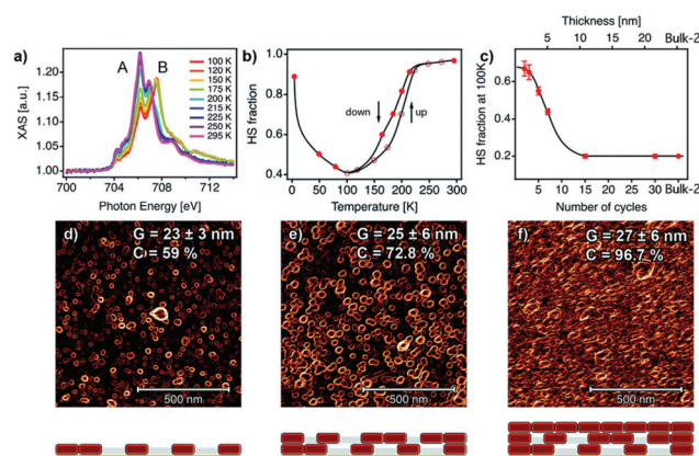
Fig. 4 (a) Temperature dependent XAS spectra for a 7-cycle [\text{Fe}(\text{py})_2\text{Pt}(\text{CN})_4] thin film; (b) temperature dependent of HS fraction for the 7-cycle film; (c) the dependence of the HS fraction on the number of cycles at 100 K; 1 \times 1 \mu\text{m}^2 AFM topography images for a (d) 2-cycles; (e) 5-cycles; (f) 10 cycles thin film. The microstructure of each film is represented below each AFM image. Adapted from ref. 28, licensed under CC BY 3.0 published by the Royal Society of Chemistry.
