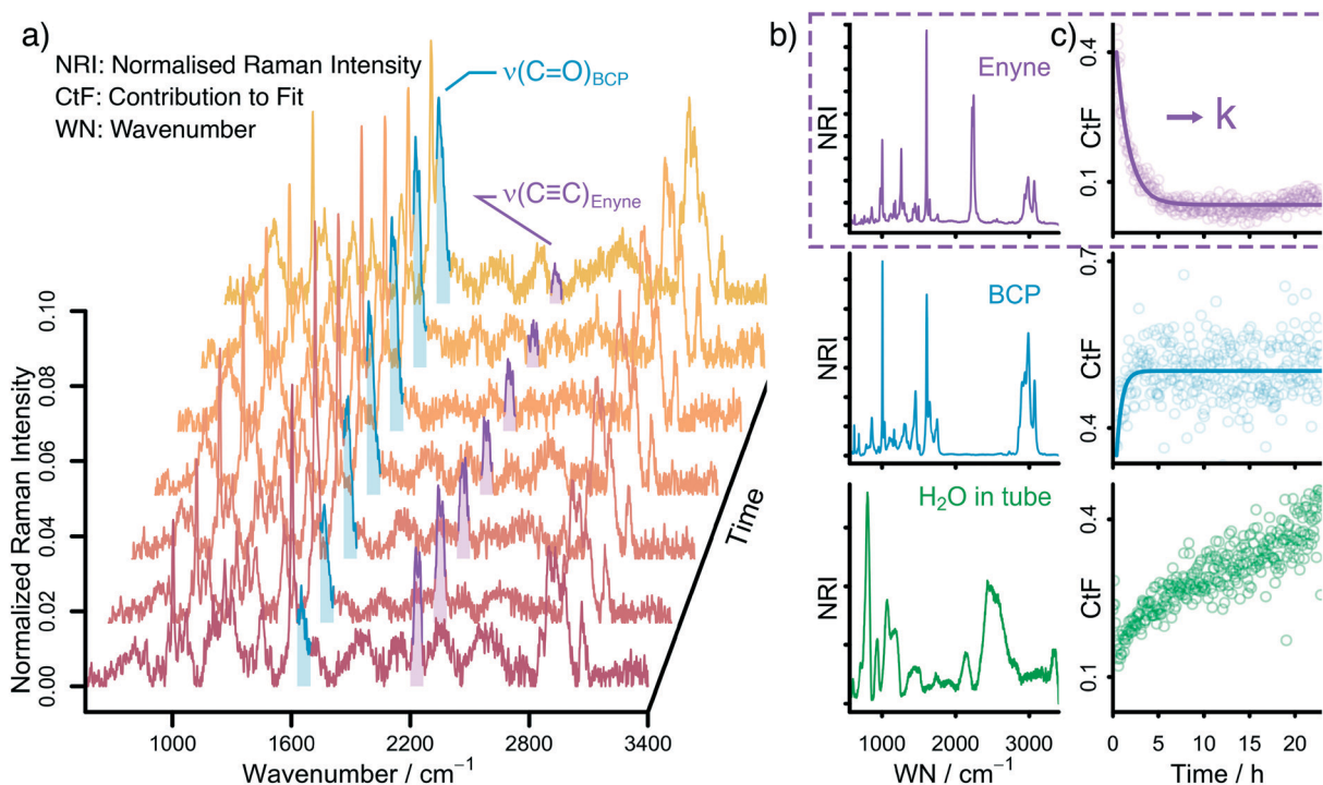
Fig. 1 a) Background-corrected and normalised in situ Raman spectra collected during the Rh-catalysed Pauson-Khand type reaction. Highlighted in purple and blue are the C≡C and C=O stretching of enyne and BCP, respectively. b) Background-corrected and normalised Raman spectra (NRI = normalised Raman intensity) of pure enyne, BCP and H 2 O in a microwave tube. These spectra are used to fit the in situ Raman spectra. c) Time-dependent contribution to the linear fit (CtF) of enyne, BCP and H 2 O. The profiles of enyne and BCP can be fitted with a first-order exponential function.
