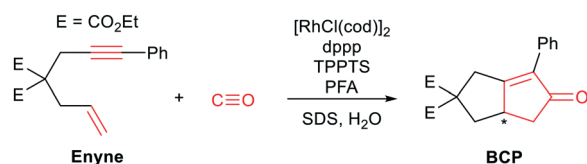
Scheme 1 Rh-Catalysed Pauson–Khand type carbonylation reaction to transform enyne components into bicyclopentenones. The functional groups participating in the cyclisation reaction are highlighted in red. The asterisk highlights the newly formed chiral centre.
