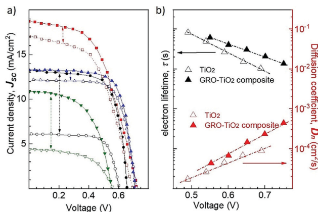
Fig. 14 (a) Typical J - V curves of DSSCs based on different GRM-based photoactive layers (line and full symbols) compared to those of the corresponding traditional \text{TiO}_2 -based photoelectrode. (b) Electron diffusion coefficient ( D_n ) and lifetime ( \tau ) dependence on the applied voltage for DSSCs based on \text{TiO}_2 photoactive layers with and without GRMs. Adapted from ref. 741,742,758,759.
