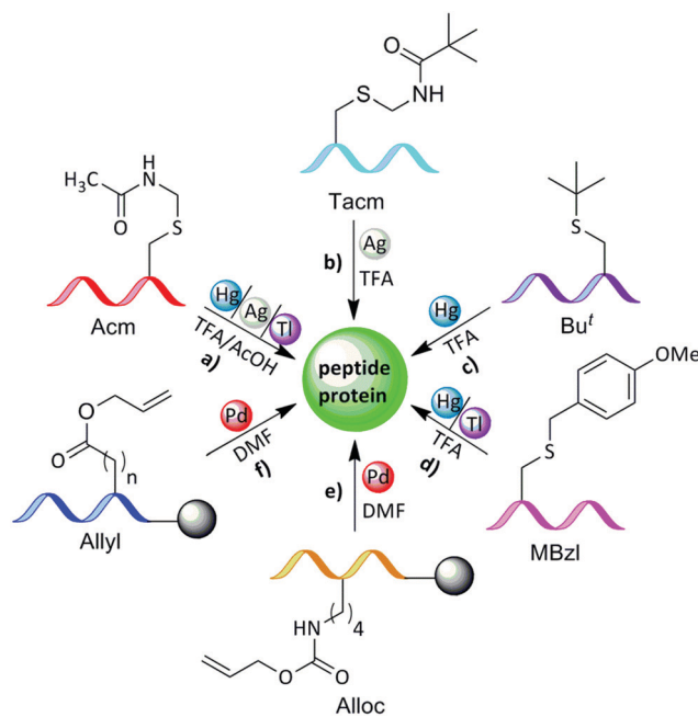
Fig. 7 Transition metal-mediated removal of the PGs in organic solvents for peptide and protein synthesis: (a) removal of Acm PG with Hg, Ag or Tl in TFA or AcOH; (b) removal of S -trimethylacetamidelmethyl (Tacm) PG with Ag in TFA; (c) removal of tert -butyl PG with Hg in TFA; (d) removal of p -methoxybenzyl (MBzl) PG with Hg or Tl in TFA; (e) removal of Alloc PG with Pd in DMF; (f) removal of allyl PG with Pd in DMF.
