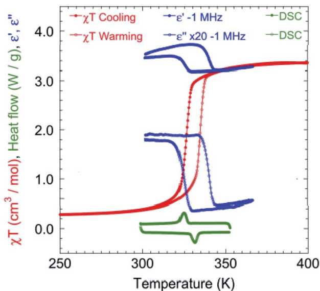
Fig. 3 Temperature dependence of \chi_{\text{MT}} in 1 kOe (red) at a rate of 2 K min −1 (see Fig. S2† for the full temperature range of \chi_{\text{MT}} ), real and imaginary ( \times 20 ) dielectricity (blue) at a rate of 20 K min −1 and DSC (green) at a rate of 15 K min −1 around the HS–LS transition.
