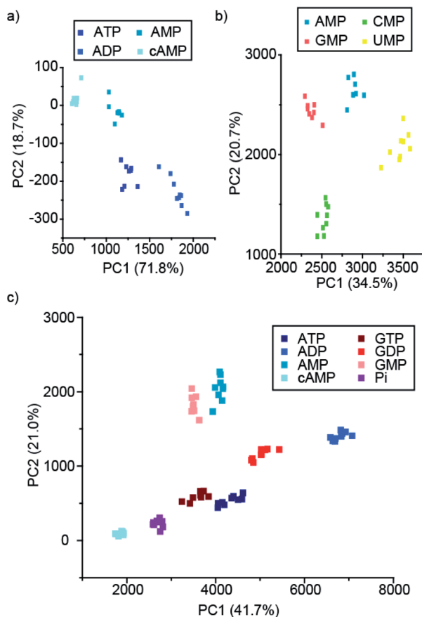
Fig. 6 PCA score plots of % change in emission intensity of (a) just [Eu.1] + (8 μM) with the adenosine series of anions (1 mM), (b) [Eu.1] + (8 μM), [Eu.2] + (13 μM), [Eu.4] + (10 μM) and [Tb.1] + (15 μM) with NMP anions (1 mM), and (c) the adenosine and guanosine series of NPP anions (1 mM), in 10 mM HEPES, pH 7.0.
