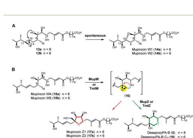
Fig. 3 (A) Structures of mupirocin W1 (14a) and W2 (14b) isolated from the \Delta mupW mutant of P. fluorescens . (B) THP ring formation in mupirocin biosynthesis catalysed by the dual action of the Rieske non-haem oxygenase MupW and the epoxide hydrolase MupZ. 14 The functions of their equivalents TmlW/TmlZ in thiomarinol biosynthesis were confirmed in the present study.
