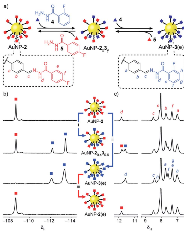
Fig. 3 Reversible dynamic covalent modification of 'electrophilic' DCNPs (surface-bound hydrazones: squares) using nucleophilic molecular modifiers (hydrazides: triangles). (a) Schematic representation of the interconversion between AuNP-2, AuNP-3 and intermediate mixed-ligand monolayer compositions AuNP- 2_x3_y . General conditions: AuNP-2 (5 mM), \text{CF}_3\text{CO}_2\text{H} (20 mM), \text{DMF}/\text{D}_2\text{O} (9 : 1 v/v), rt. (b) Partial ^{19}\text{F} NMR spectra ( [\text{D}_7]\text{DMF} , 470 MHz, 295 K, internal standard: \text{CFCl}_3 ). (c) Partial ^1\text{H} NMR spectra ( [\text{D}_7]\text{DMF} , 500 MHz, 295 K). Spectra from top to bottom: AuNP-2 (direct synthesis); AuNP- 2_{0.4}3_{0.6} (conditions (i): 1.0 eq. 4, 1 h); AuNP-3(e) (conditions (ii): 25 eq. 4, 1.2 h); AuNP-2(e) (conditions (iii): 25 eq. 5, 2.2 h). Full sweep-width spectra and pre-purification spectra can be found in Fig. S15–S17 and S21. †
