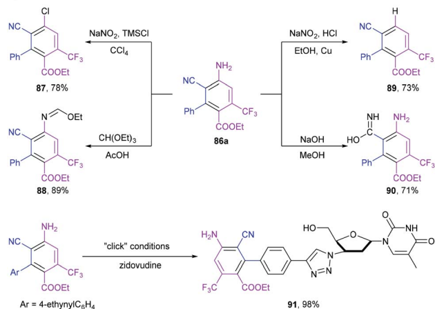
Scheme 25 DABCO-catalyzed [4 + 2] benzannulation to synthesize biaryls.
