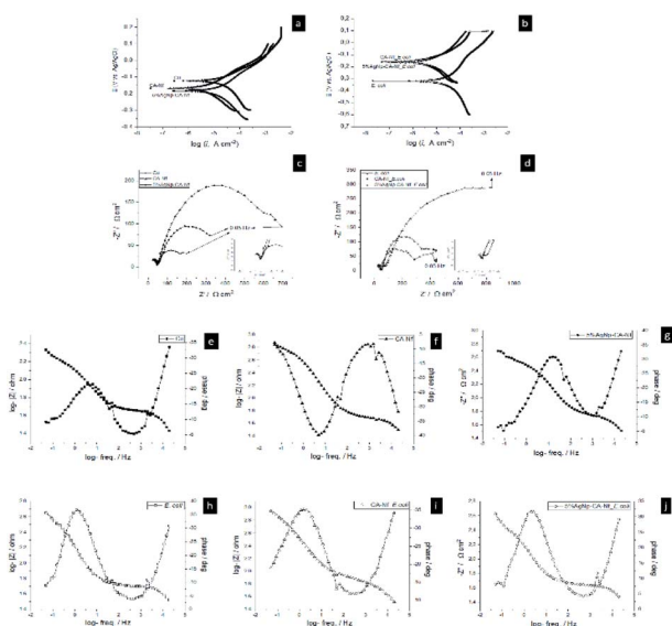
Fig. 9 Abiotic and biotic corrosion set ups potentiodynamic polarization curves (a and b), Nyquist plots (c and d) and Bode plots (e-j).
